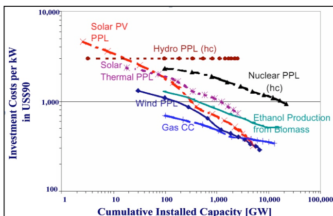
Figure 3. The greater the installed capacity of an energy technology, the lower price for every new unit installed. (Source: Nakicenovic, IIASA, 2009)
