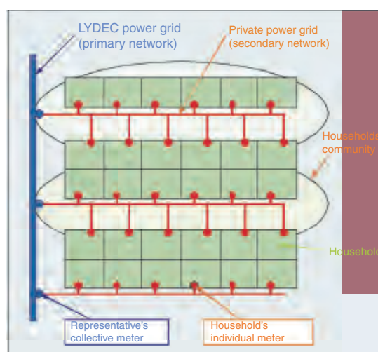
Slum electrification 2 layered network: LYDEC's owned network in blue, private community network in red
